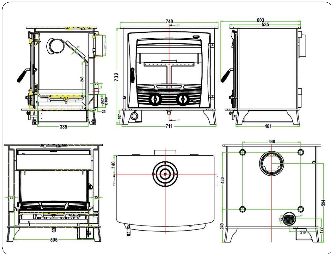
Druid 30 Boiler
