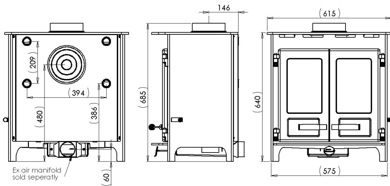
Inis Oirr MK2 Boiler/Roomheater
